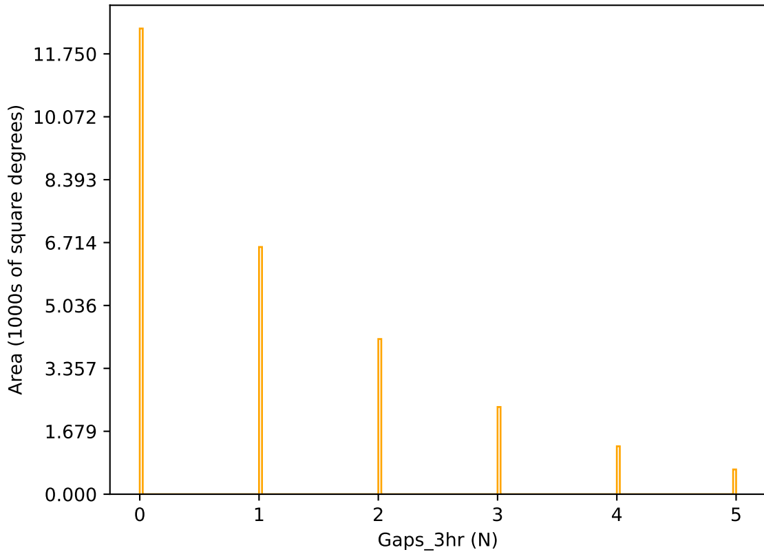
weather_cloudso18v3.4_10yrs r band: Gaps_3hr
