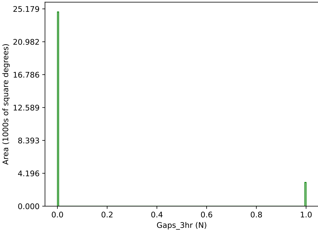
weather_cloudso18v3.4_10yrs g band: Gaps_3hr
