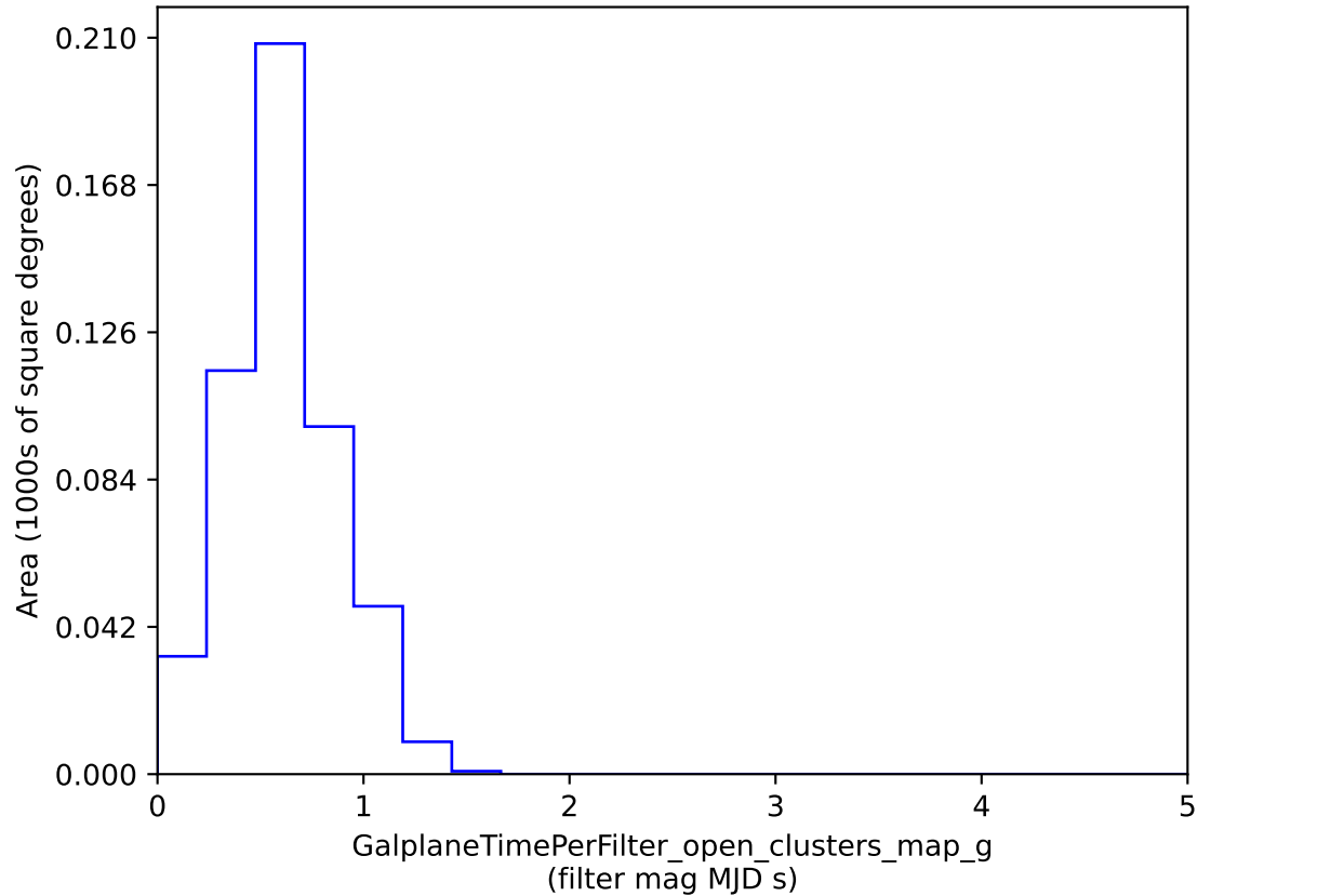
weather_cloudso18v3.4_10yrs : GalplaneTimePerFilter_open_clusters_map_g
