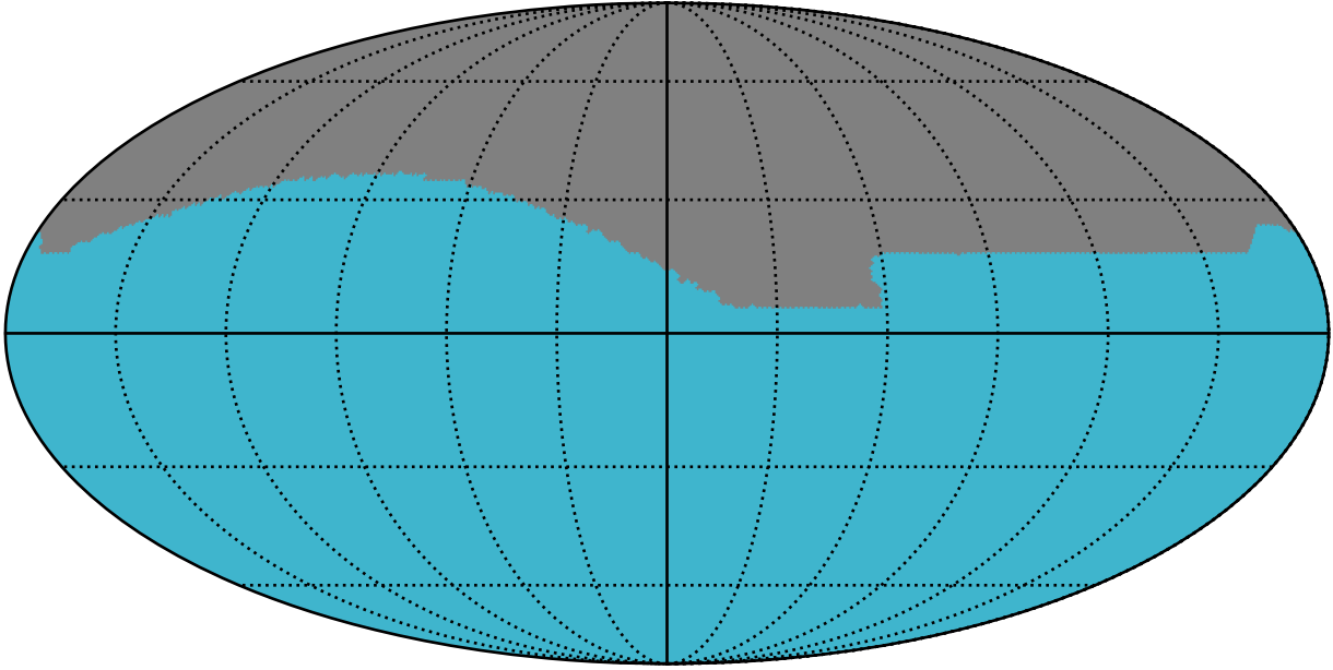
weather_cloudso18v3.4_10yrs : GalplaneFootprintMetric_xray_binaries_map_Tau_2_0
