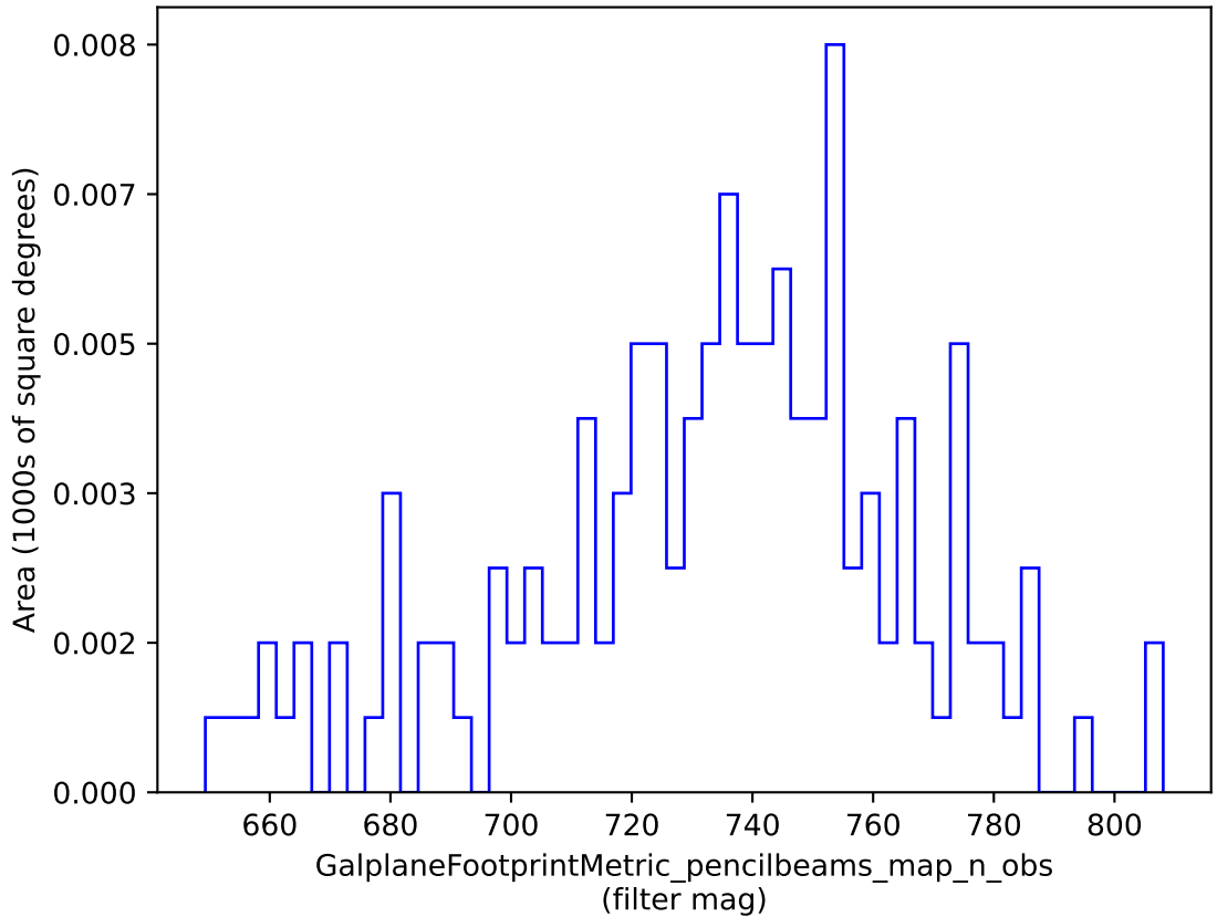
weather_cloudso18v3.4_10yrs : GalplaneFootprintMetric_pencilbeams_map_n_obs
