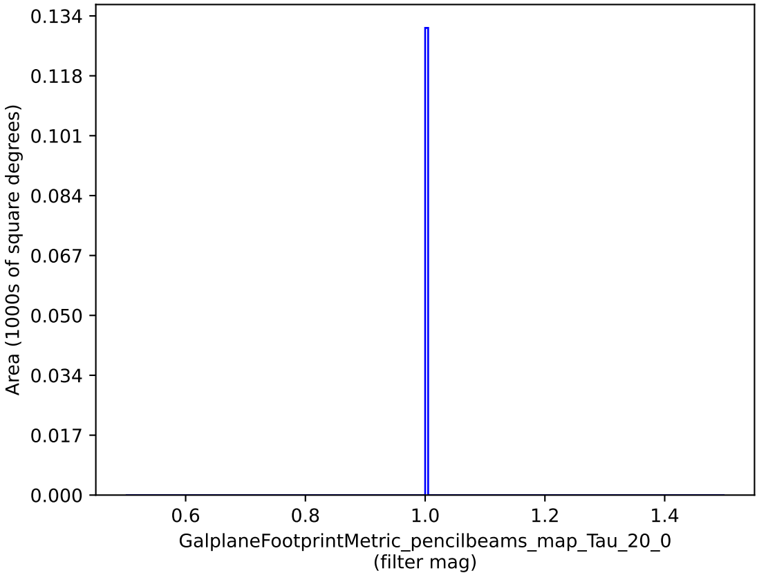
weather_cloudso18v3.4_10yrs : GalplaneFootprintMetric_pencilbeams_map_Tau_20_0
