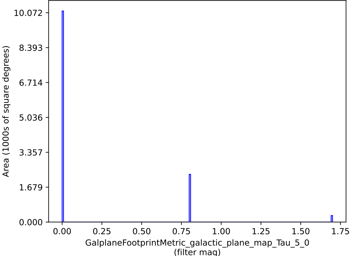
weather_cloudso18v3.4_10yrs : GalplaneFootprintMetric_galactic_plane_map_Tau_5_0
