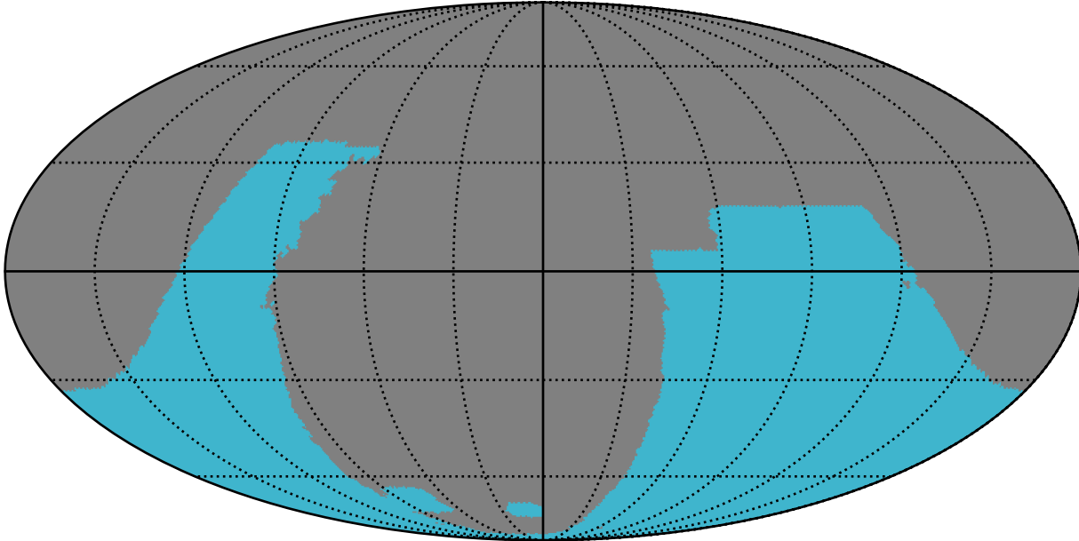
weather_cloudso18v3.4_10yrs : GalplaneFootprintMetric_galactic_plane_map_Tau_2_0
