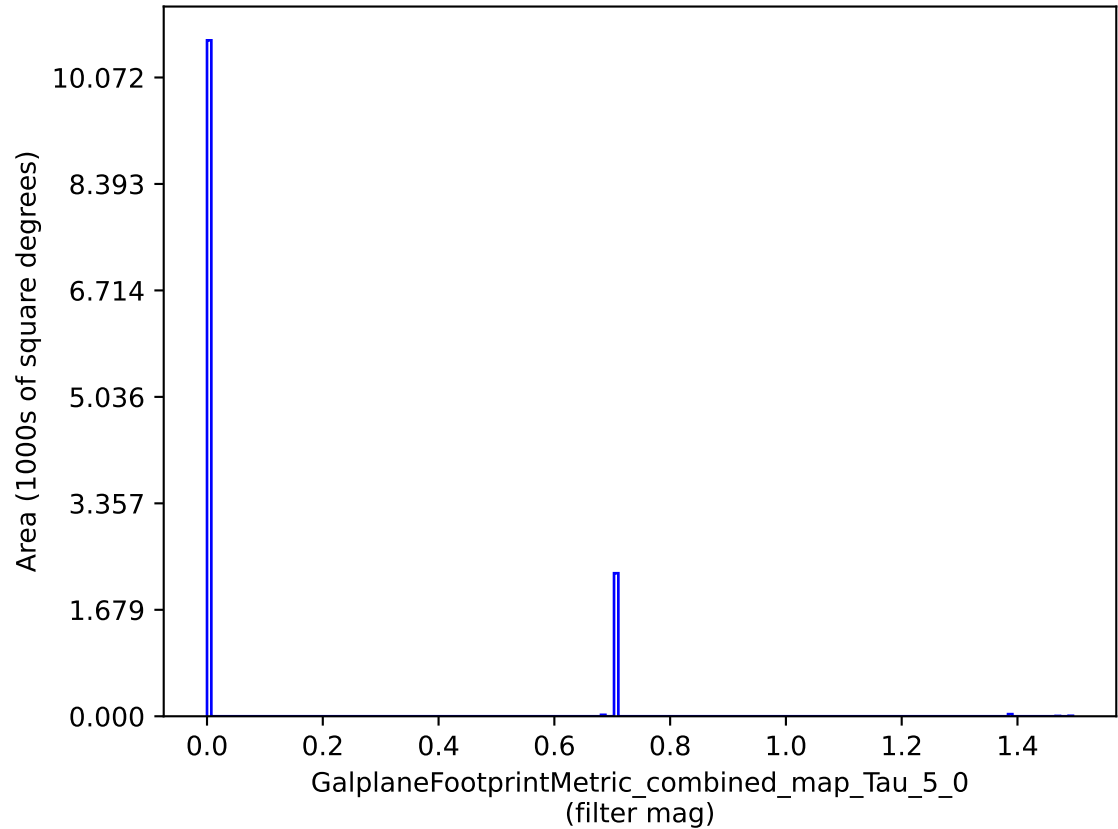
weather_cloudso18v3.4_10yrs : GalplaneFootprintMetric_combined_map_Tau_5_0
