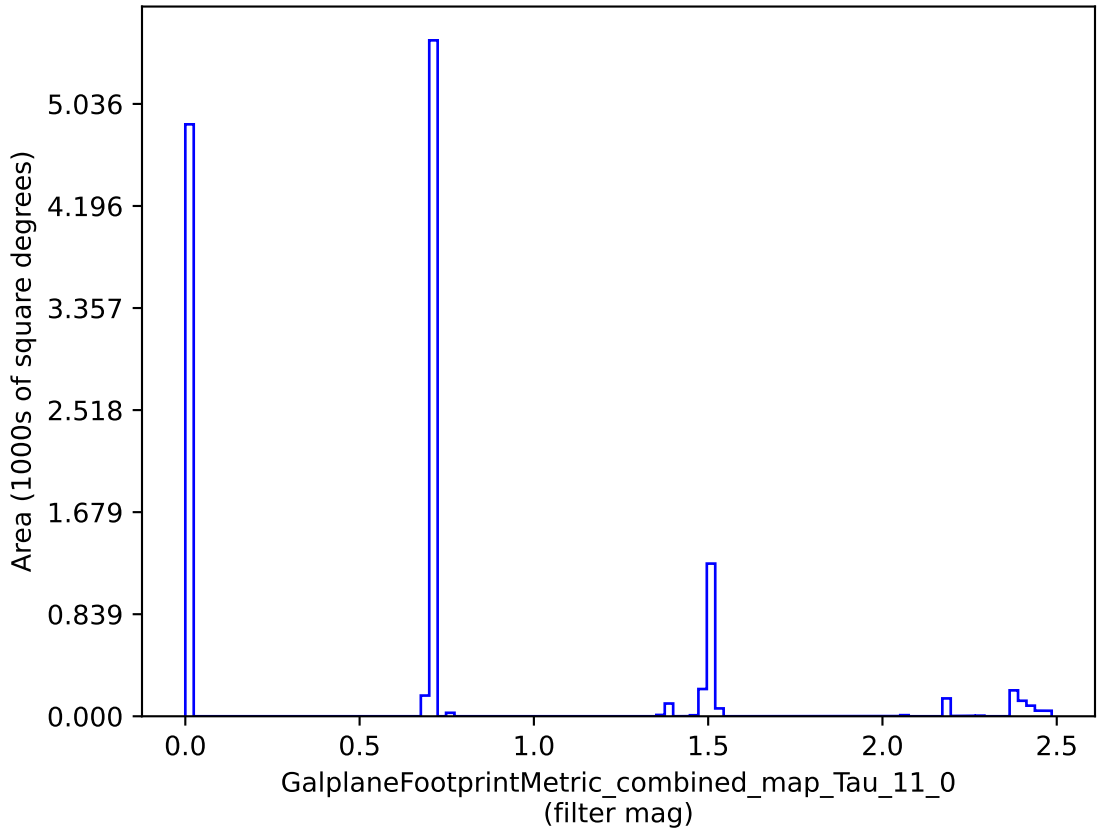
weather_cloudso18v3.4_10yrs : GalplaneFootprintMetric_combined_map_Tau_11_0
