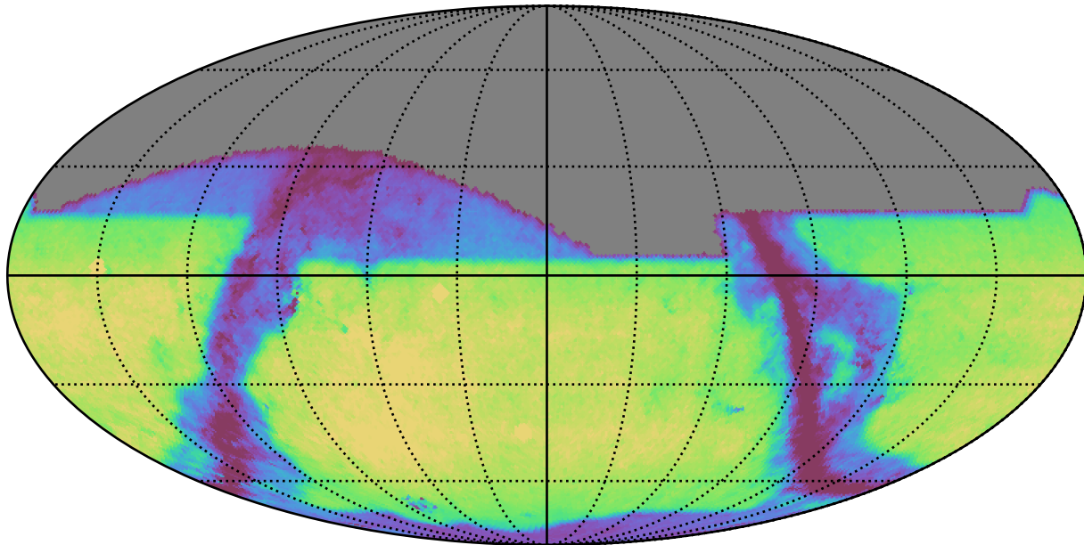
weather_cloudso18v3.4_10yrs z: GalaxyCountsMetricExtended
