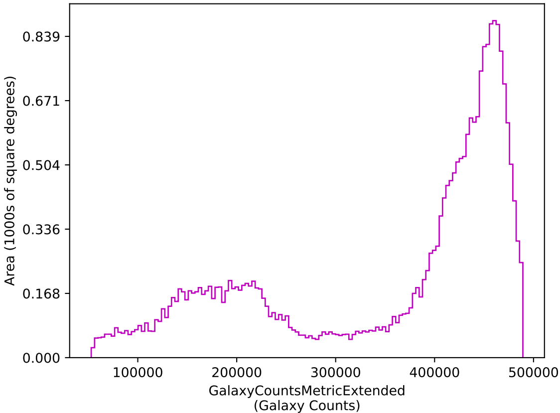
weather_cloudso18v3.4_10yrs z: GalaxyCountsMetricExtended
