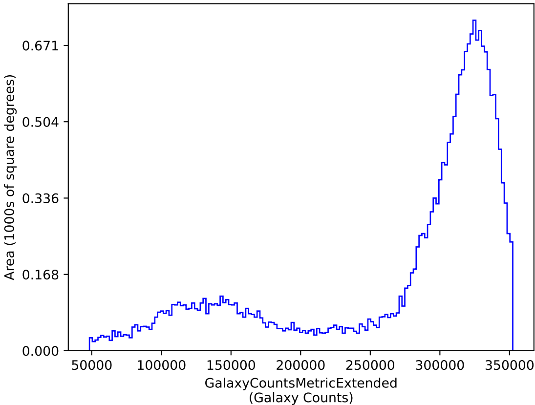
weather_cloudso18v3.4_10yrs y: GalaxyCountsMetricExtended
