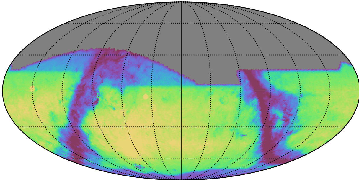
weather_cloudso18v3.4_10yrs r: GalaxyCountsMetricExtended
