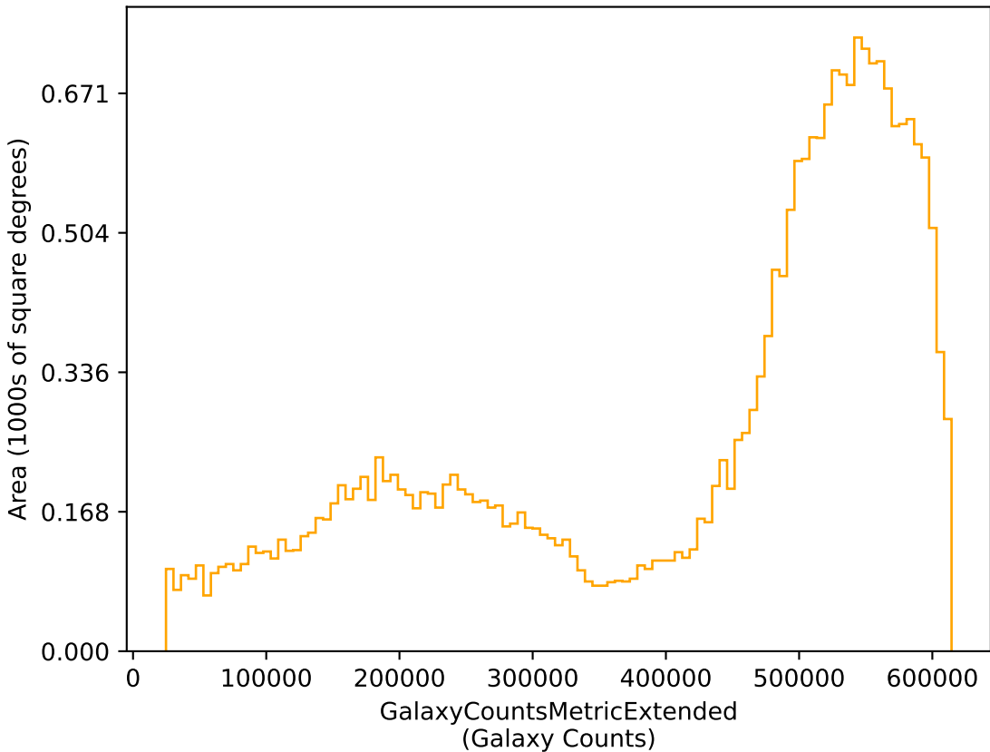
weather_cloudso18v3.4_10yrs r: GalaxyCountsMetricExtended
