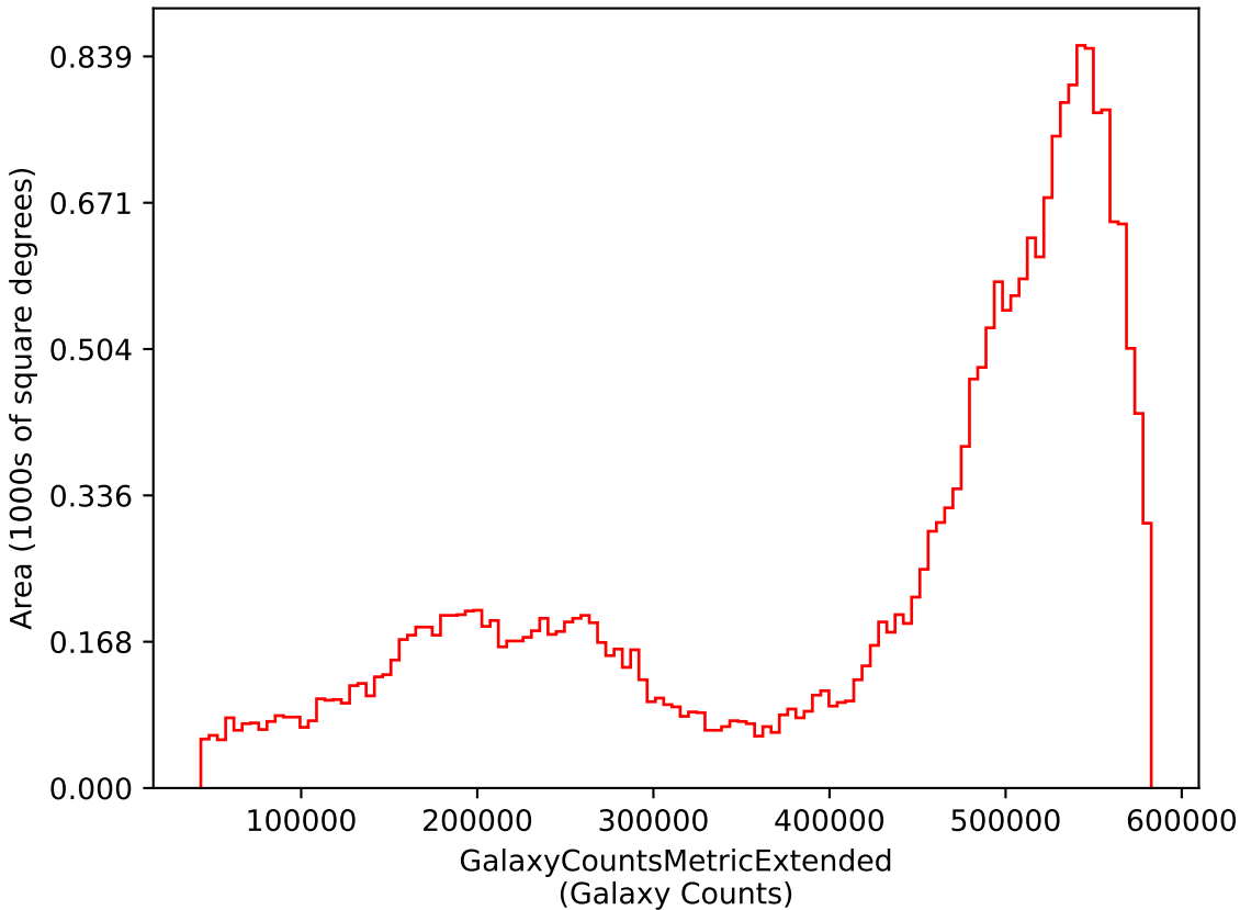
weather_cloudso18v3.4_10yrs i: GalaxyCountsMetricExtended
