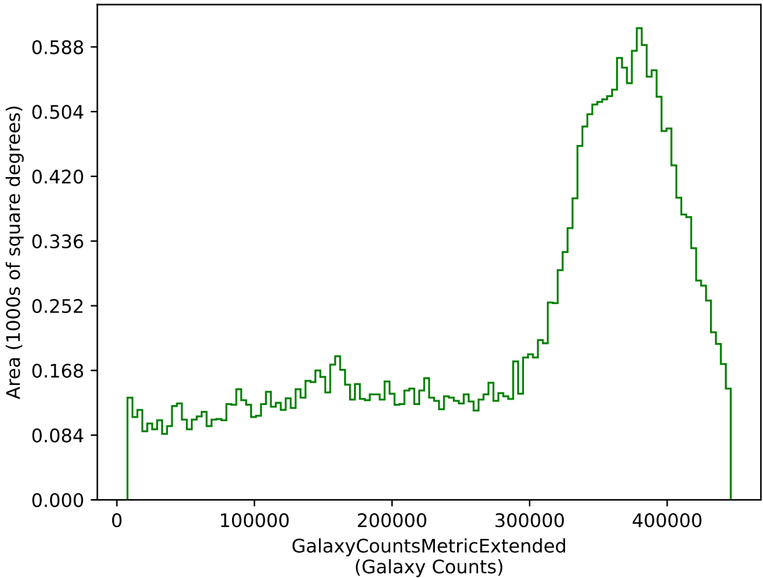
weather_cloudso18v3.4_10yrs g: GalaxyCountsMetricExtended
