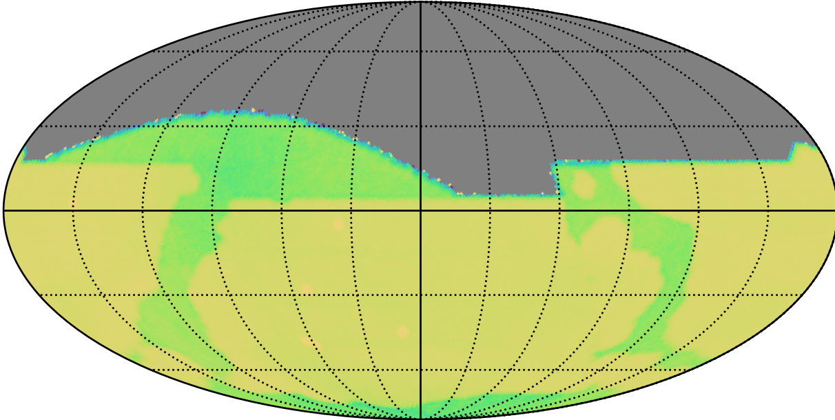
weather_cloudso18v3.4_10yrs : GalPlaneVisitIntervalsTimescales_xray_binaries_map_Tau_11_0
