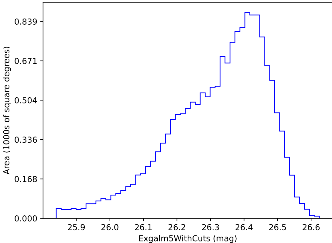
weather_cloudso18v3.4_10yrs i band non-DD year 9: ExgalM5WithCuts
