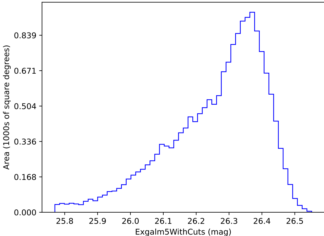
weather_cloudso18v3.4_10yrs i band non-DD year 8: ExgalM5WithCuts
