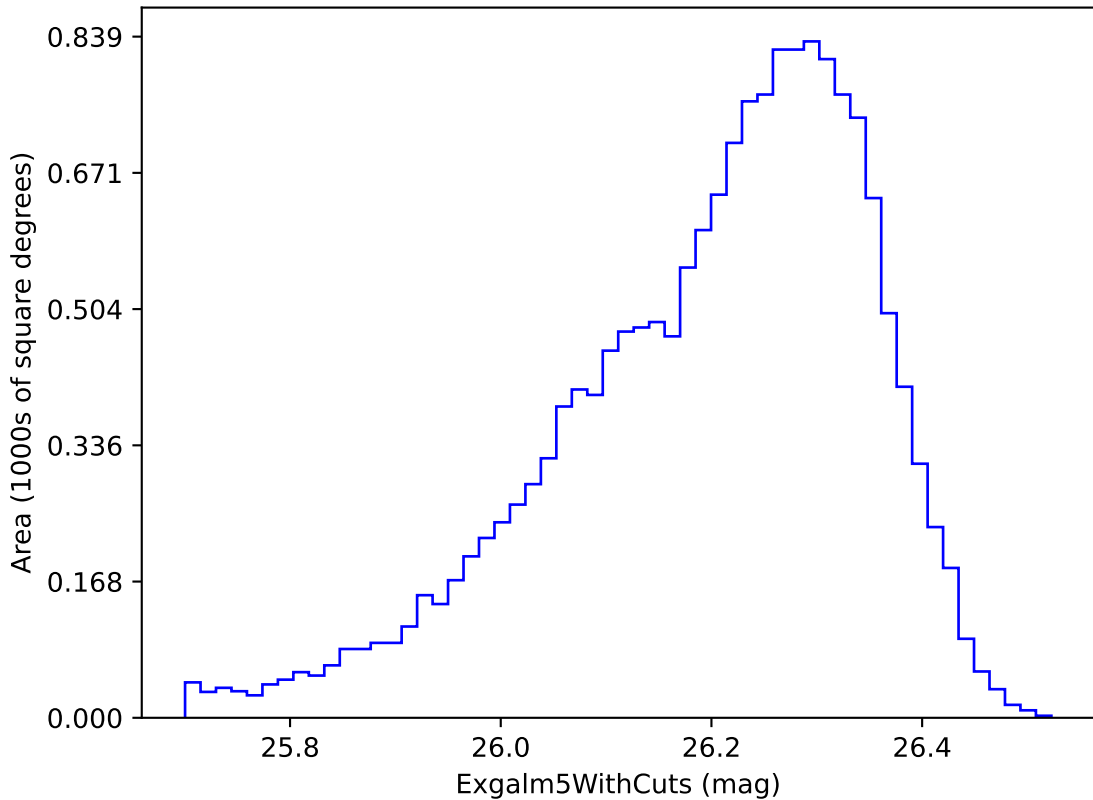
weather_cloudso18v3.4_10yrs i band non-DD year 7: ExgalM5WithCuts
