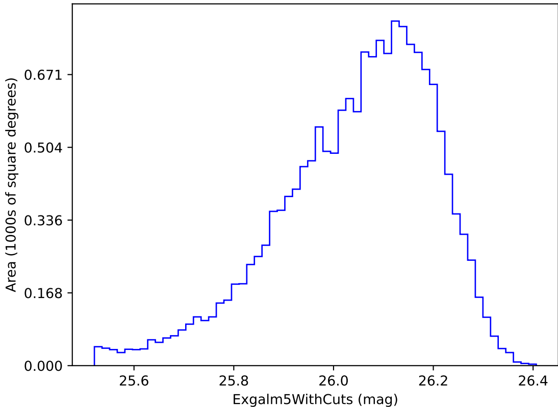
weather_cloudso18v3.4_10yrs i band non-DD year 5: ExgalM5WithCuts
