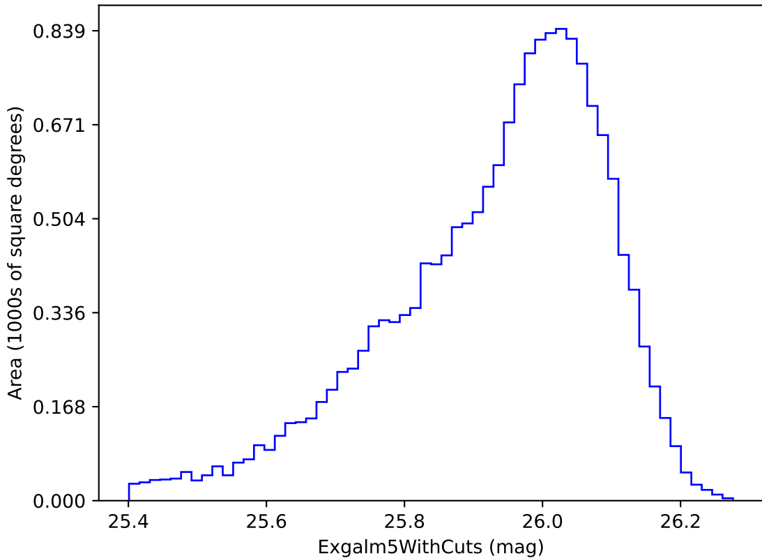
weather_cloudso18v3.4_10yrs i band non-DD year 4: ExgalM5WithCuts
