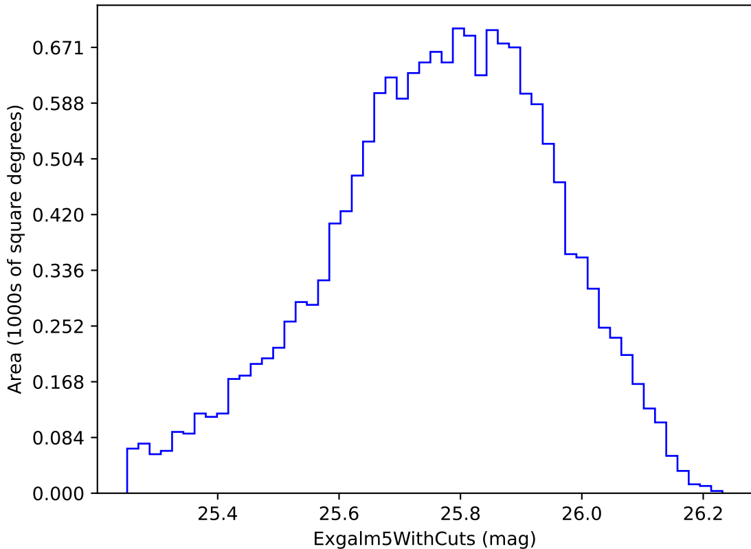
weather_cloudso18v3.4_10yrs i band non-DD year 3: Exgalml5WithCuts
