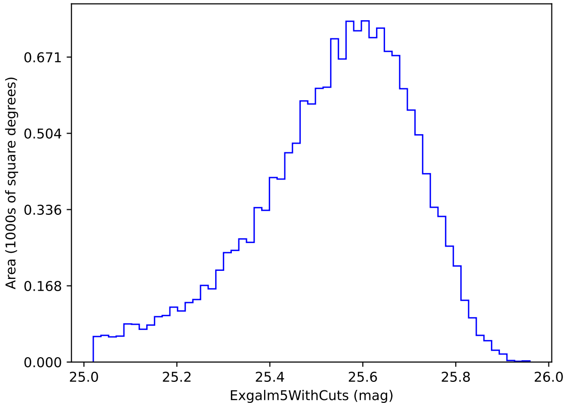
weather_cloudso18v3.4_10yrs i band non-DD year 2: ExgalM5WithCuts
