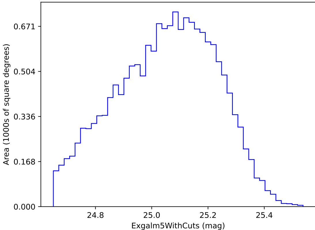
weather_cloudso18v3.4_10yrs i band non-DD year 1: ExgalM5WithCuts
