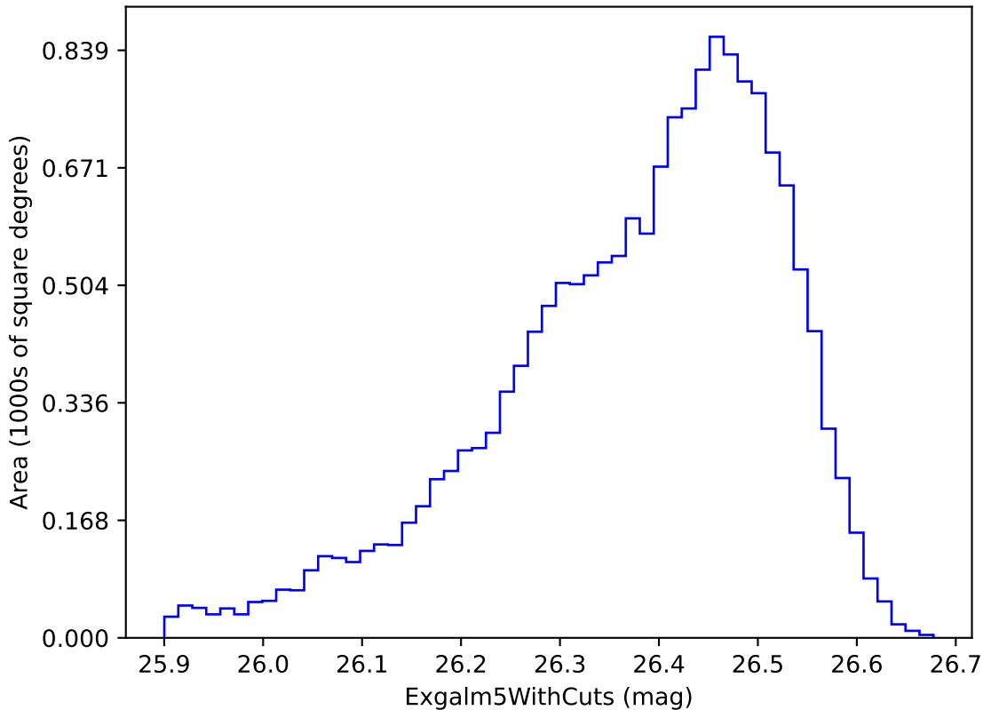
weather_cloudso18v3.4_10yrs i band non-DD year 10: Exgalml5WithCuts
