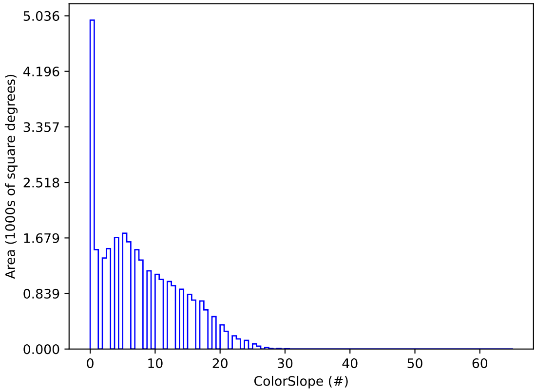
weather_cloudso18v3.4_10yrs visitExposureTime > 19: ColorSlope
