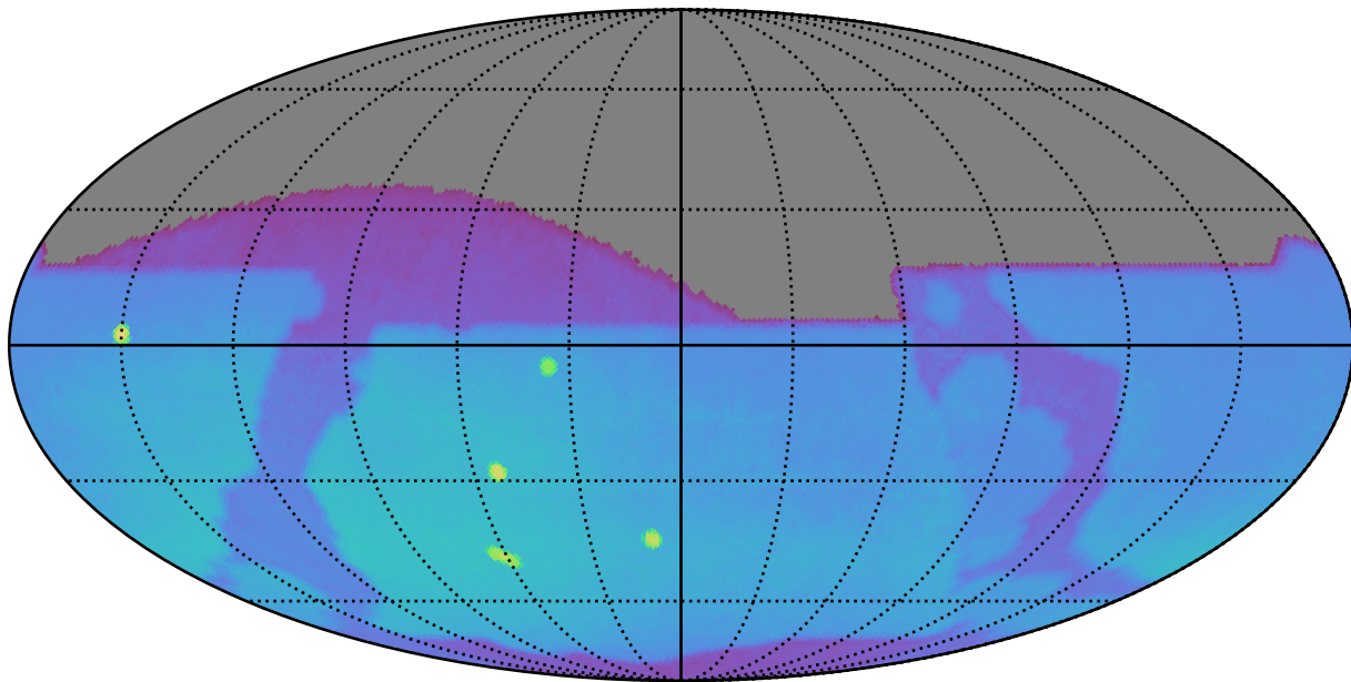
weather_cloudso18v3.4_10yrs : Brown Dwarf, L7
