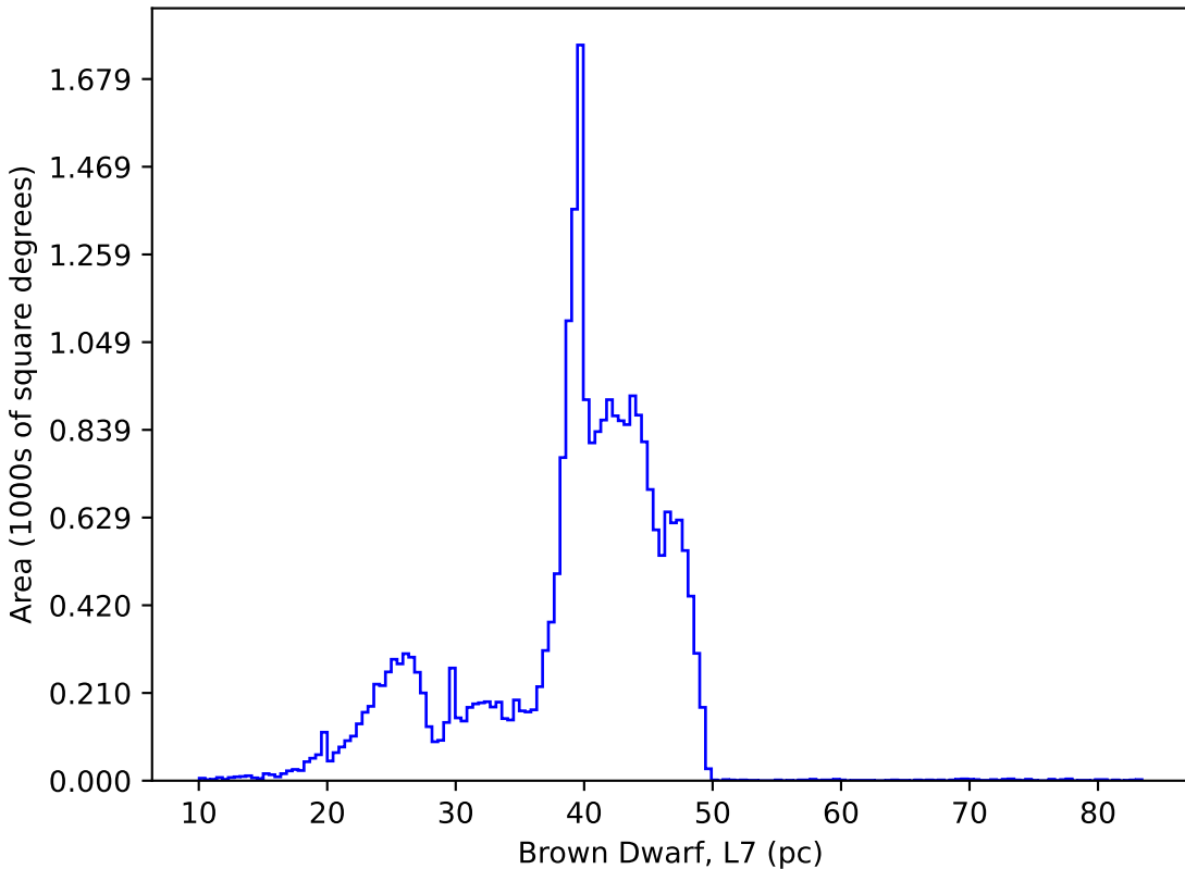
weather_cloudso18v3.4_10yrs : Brown Dwarf, L7
