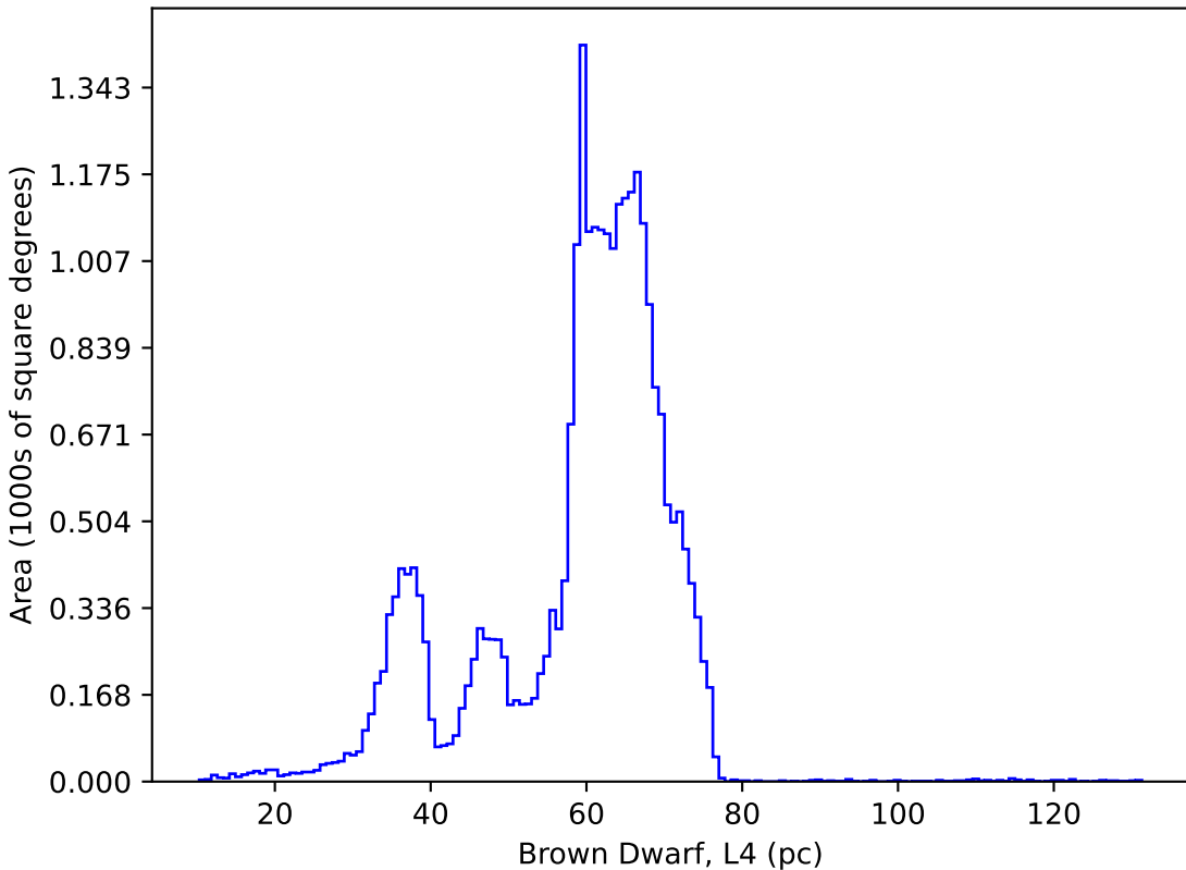
weather_cloudso18v3.4_10yrs : Brown Dwarf, L4
