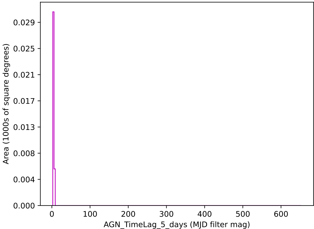
weather_cloudso18v3.4_10yrs z band: AGN_TimeLag_5_days
