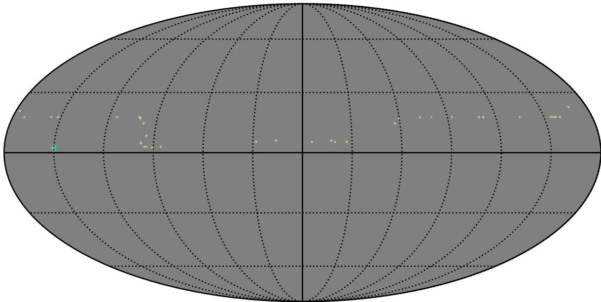
weather_cloudso18v3.4_10yrs y band: AGN_TimeLag_5_days
