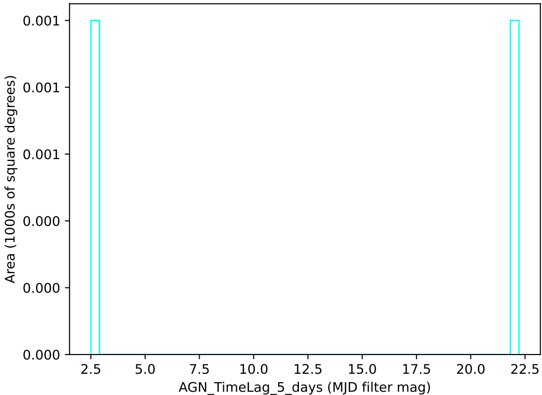
weather_cloudso18v3.4_10yrs u band: AGN_TimeLag_5_days
