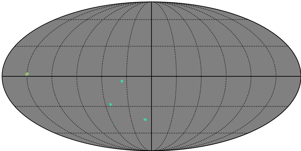
weather_cloudso18v3.4_10yrs r band: AGN_TimeLag_5_days
