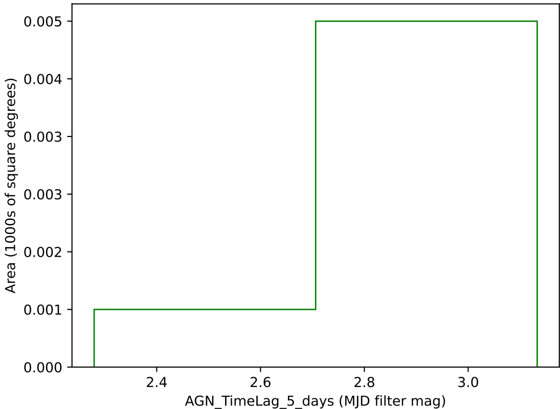
weather_cloudso18v3.4_10yrs g band: AGN_TimeLag_5_days
