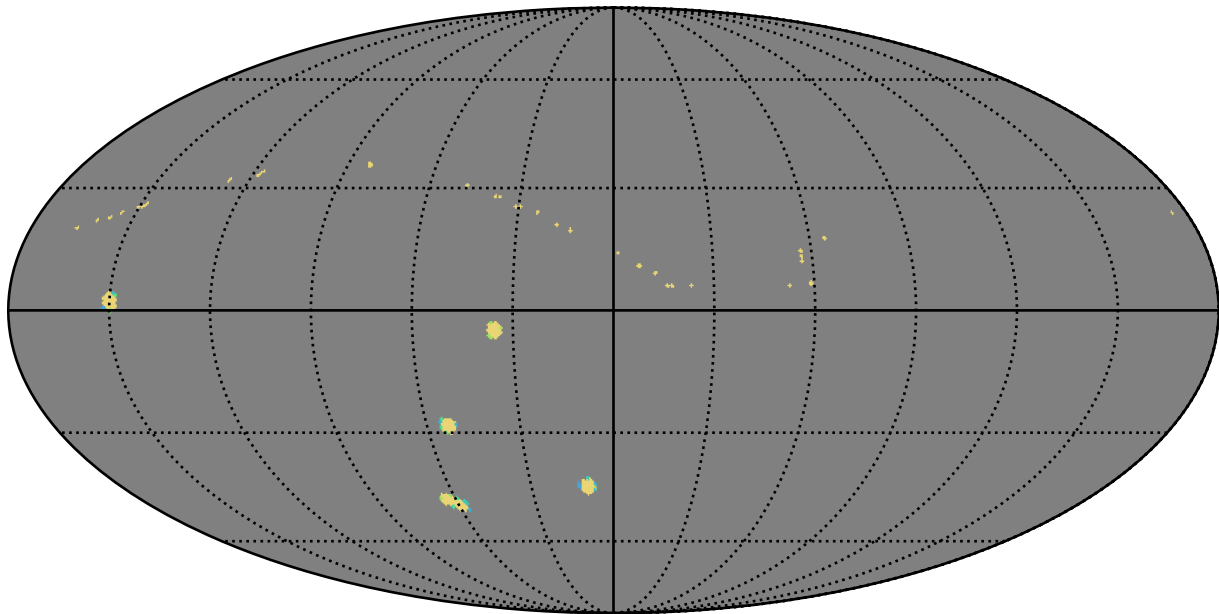
weather_cloudso18v3.4_10yrs all bands: AGN_TimeLag_5_days
