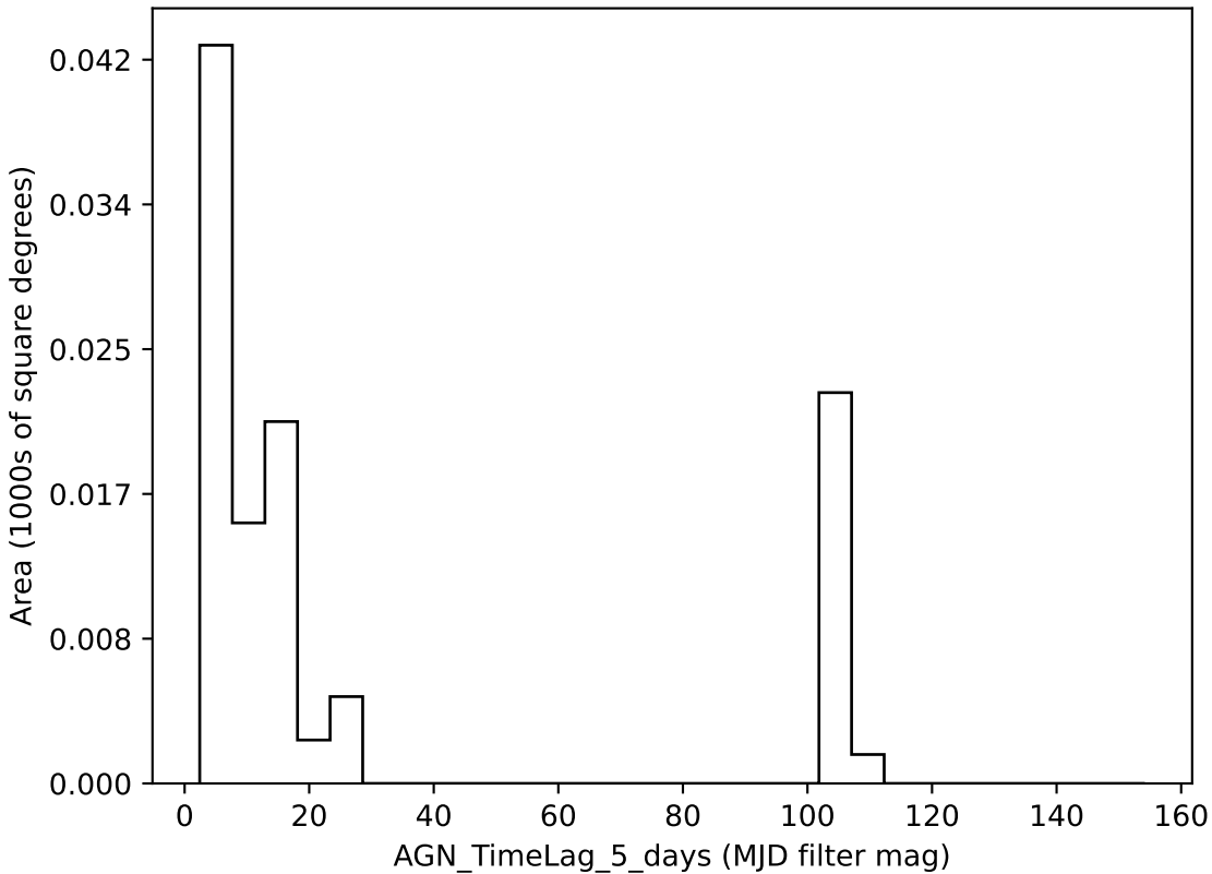
weather_cloudso18v3.4_10yrs all bands: AGN_TimeLag_5_days
