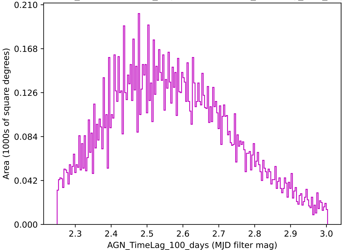
weather_cloudso18v3.4_10yrs z band: AGN_TimeLag_100_days
