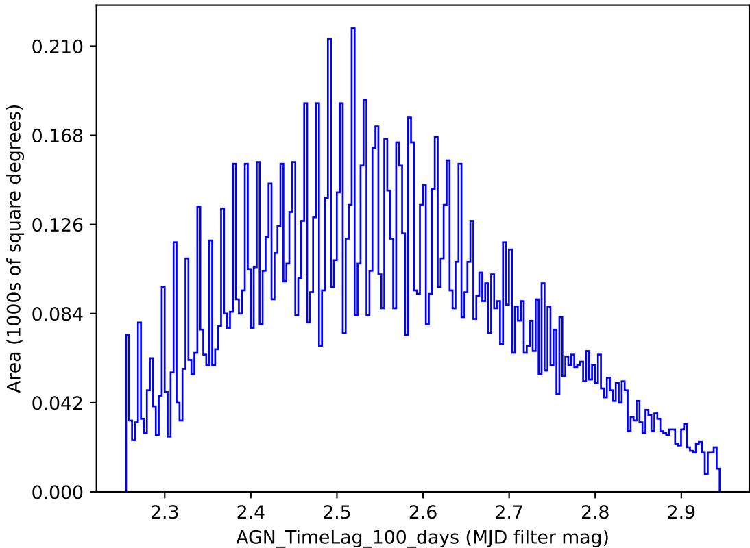
weather_cloudso18v3.4_10yrs y band: AGN_TimeLag_100_days
