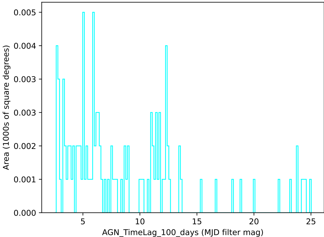
weather_cloudso18v3.4_10yrs u band: AGN_TimeLag_100_days
