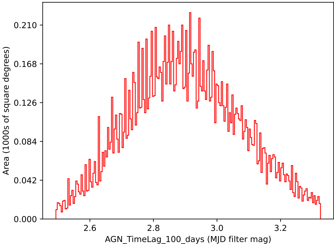
weather_cloudso18v3.4_10yrs i band: AGN_TimeLag_100_days
