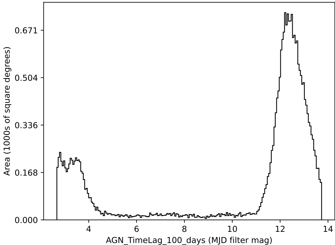
weather_cloudso18v3.4_10yrs all bands: AGN_TimeLag_100_days
