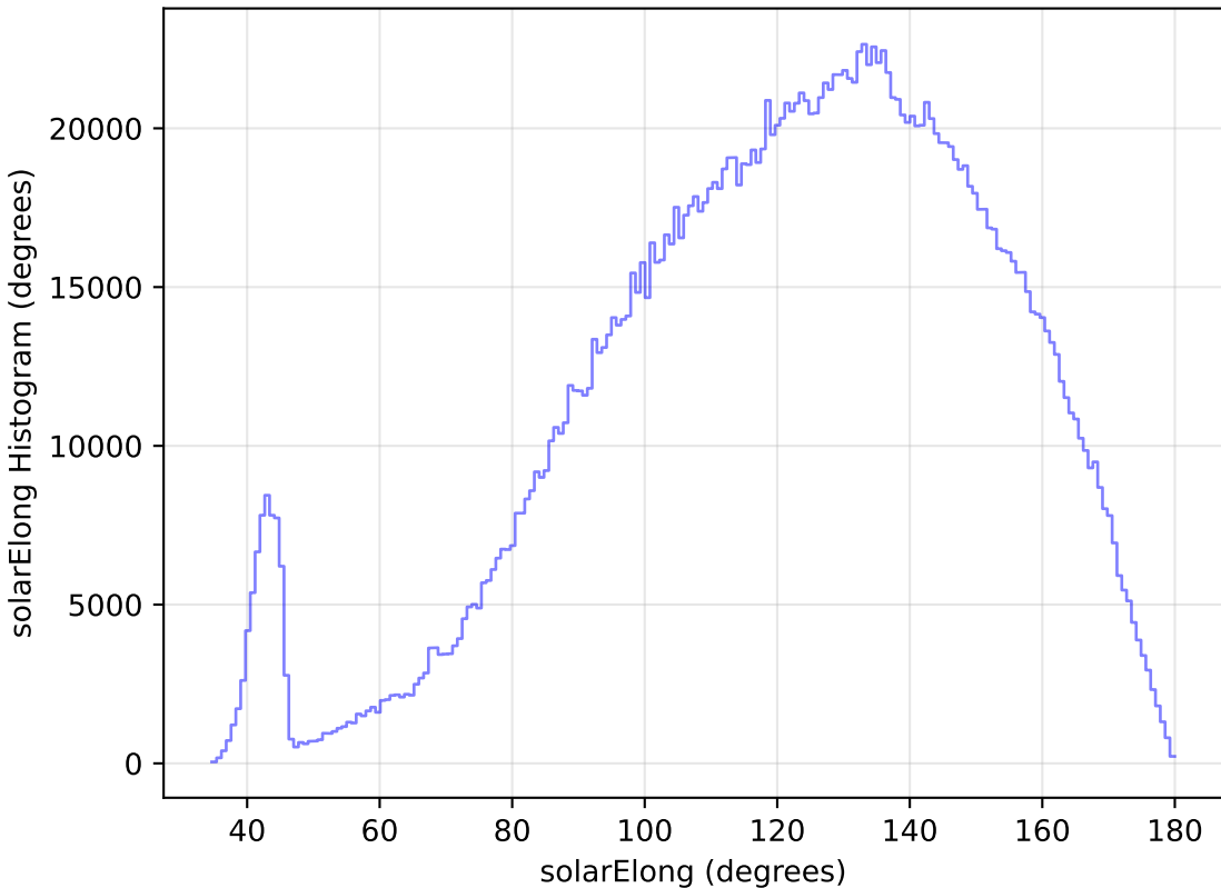
weather_cloudso18v3.4_10yrs WFD all bands: solarElong Histogram
