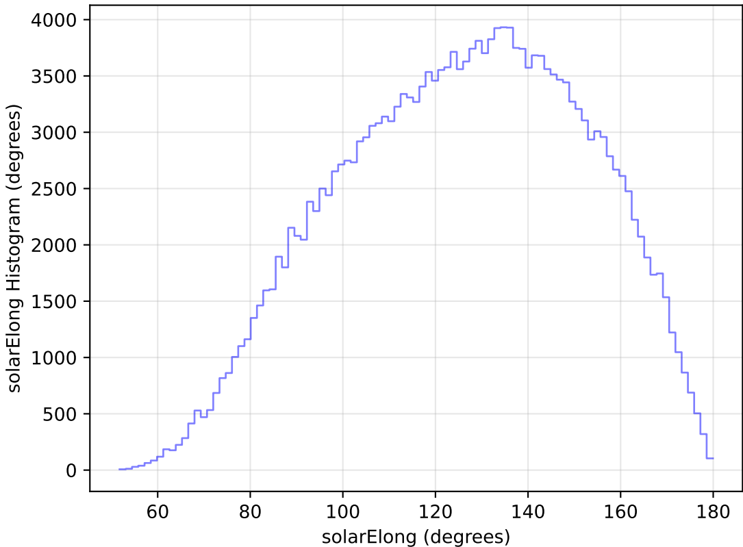
weather_cloudso18v3.4_10yrs All sky g band: solarElong Histogram
