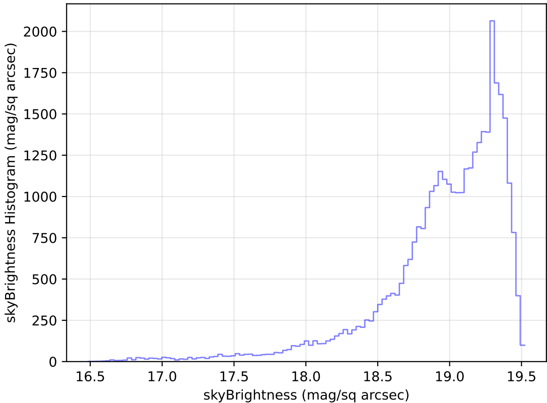
weather_cloudso18v3.4_10yrs Yr 1 z band: skyBrightness Histogram
