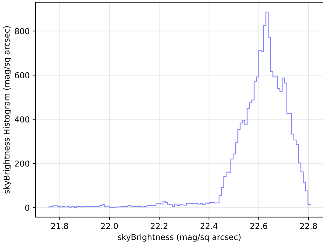
weather_cloudso18v3.4_10yrs Yr 1 u band: skyBrightness Histogram
