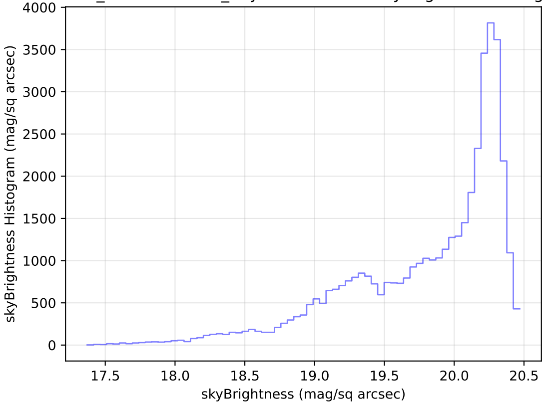
weather_cloudso18v3.4_10yrs Yr 1 i band: skyBrightness Histogram
