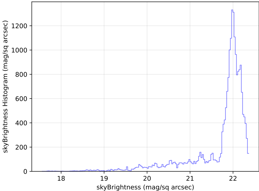
weather_cloudso18v3.4_10yrs Yr 1 g band: skyBrightness Histogram
