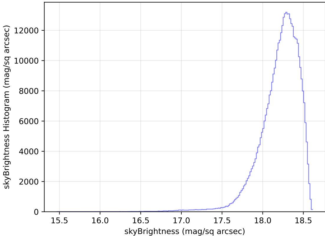
weather_cloudso18v3.4_10yrs WFD y band: skyBrightness Histogram
